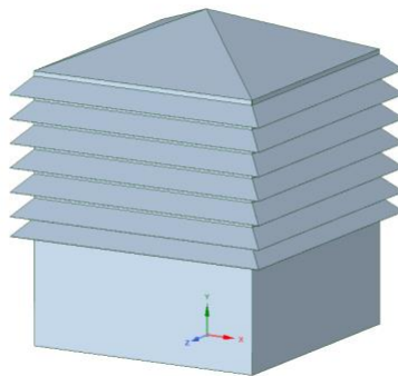
Figure 2 CAD representation of the wind tower.
