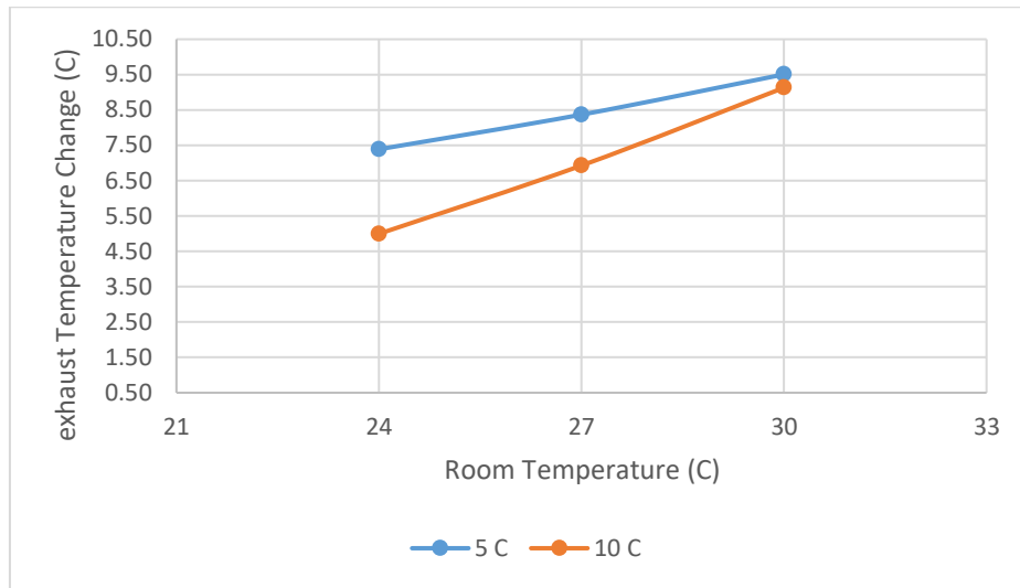
Figure 10 Exhaust temperature change for 4 ms -1 wind speed.
