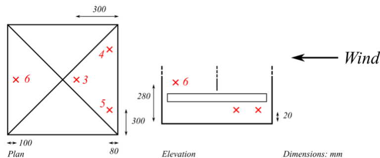
Figure 6 Location of the wind tower internal measuring points.
