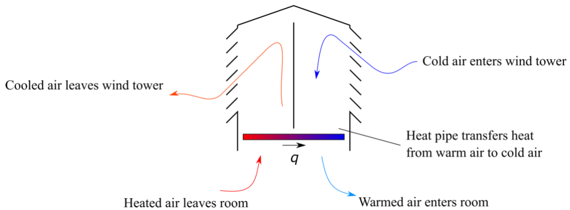
Figure 1 Schematic of wind tower heat recovery using heat pipes.
