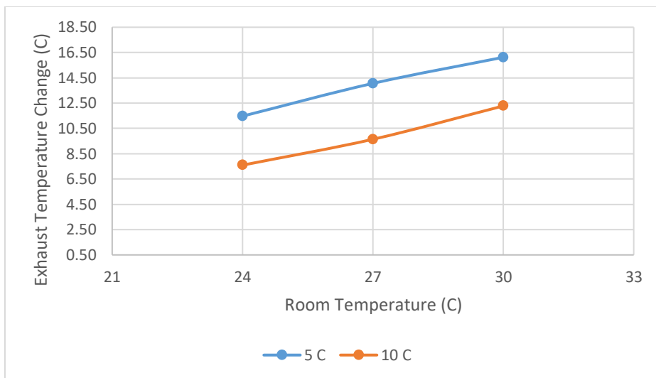
Figure 9 Exhaust temperature change for 2 ms -1 wind speed.
