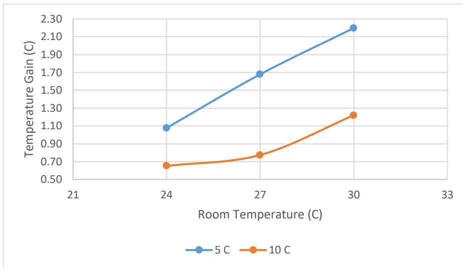
Figure 8 Temperature gain to the incoming air for 4 ms -1 wind speed.
