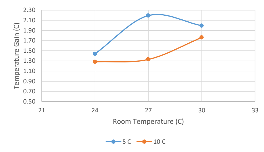
Figure 7 Temperature gain to the incoming air for 2 ms -1 wind speed.
