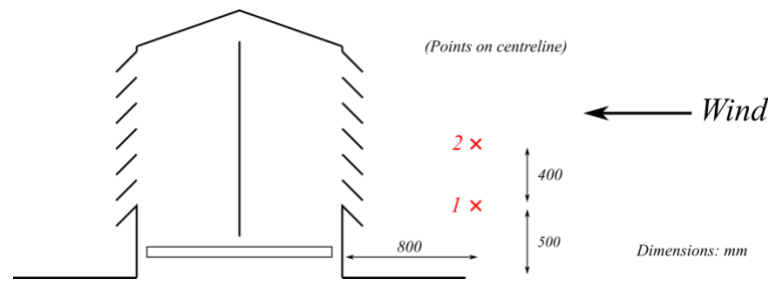
Figure 5 Location of the external measuring points.
